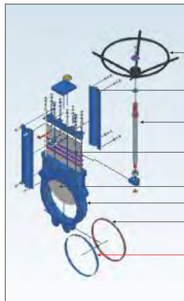
Exploded view of ZFI-S valves
