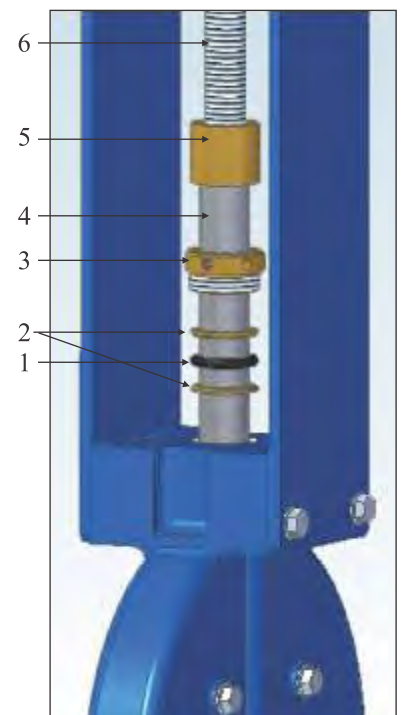
View showing glandless design feature
