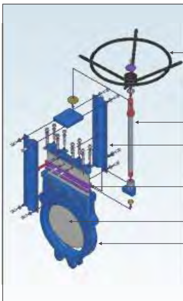
Exploded view of ZFI-M valves
